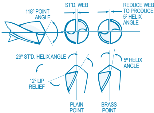
Figure 1: Drill Configuration
