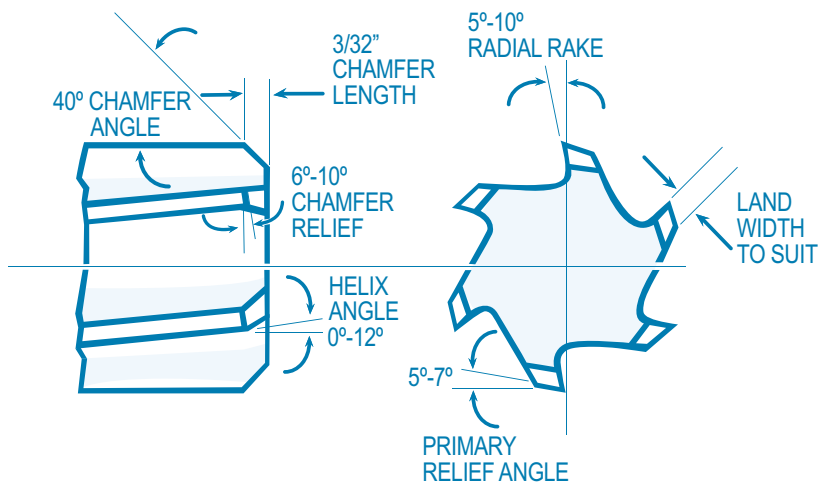
Figure 3: Reamer Configuration
